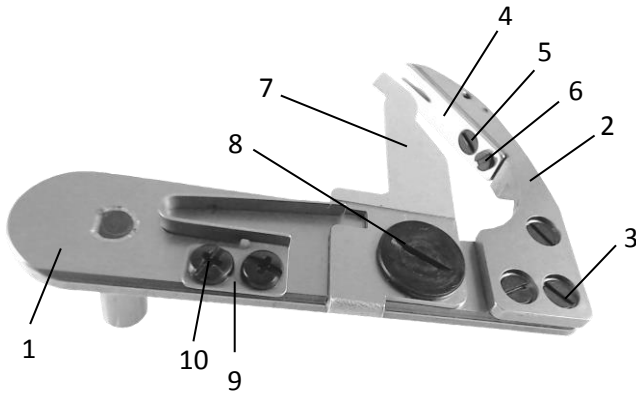
RH-9820-1 MOVABLE KNIFE HOLDER ASSEMBLY
