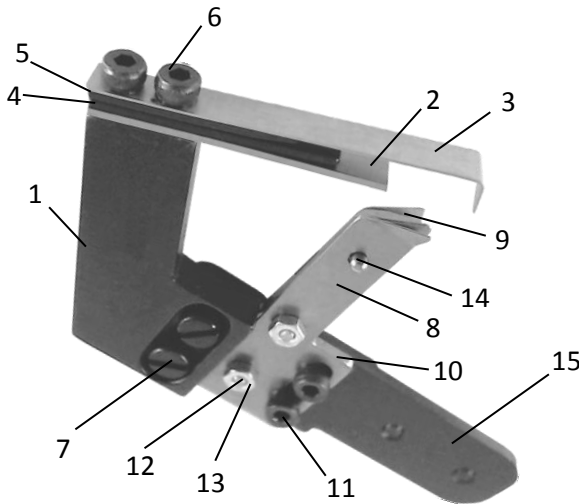
RH-9820-2 FIXED KNIFE HOLDER ASSEMBLY
